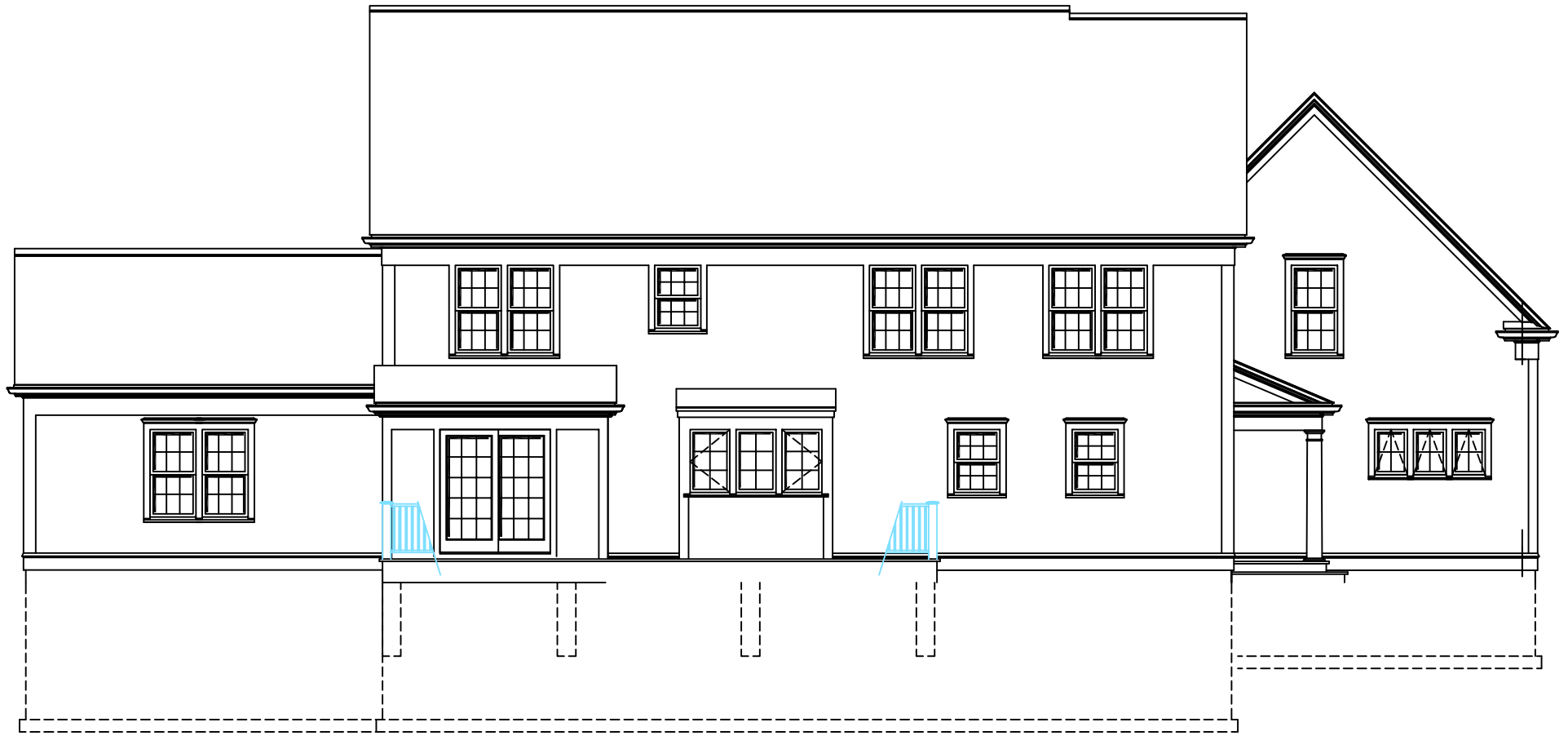
○ REAR ELEVATION
