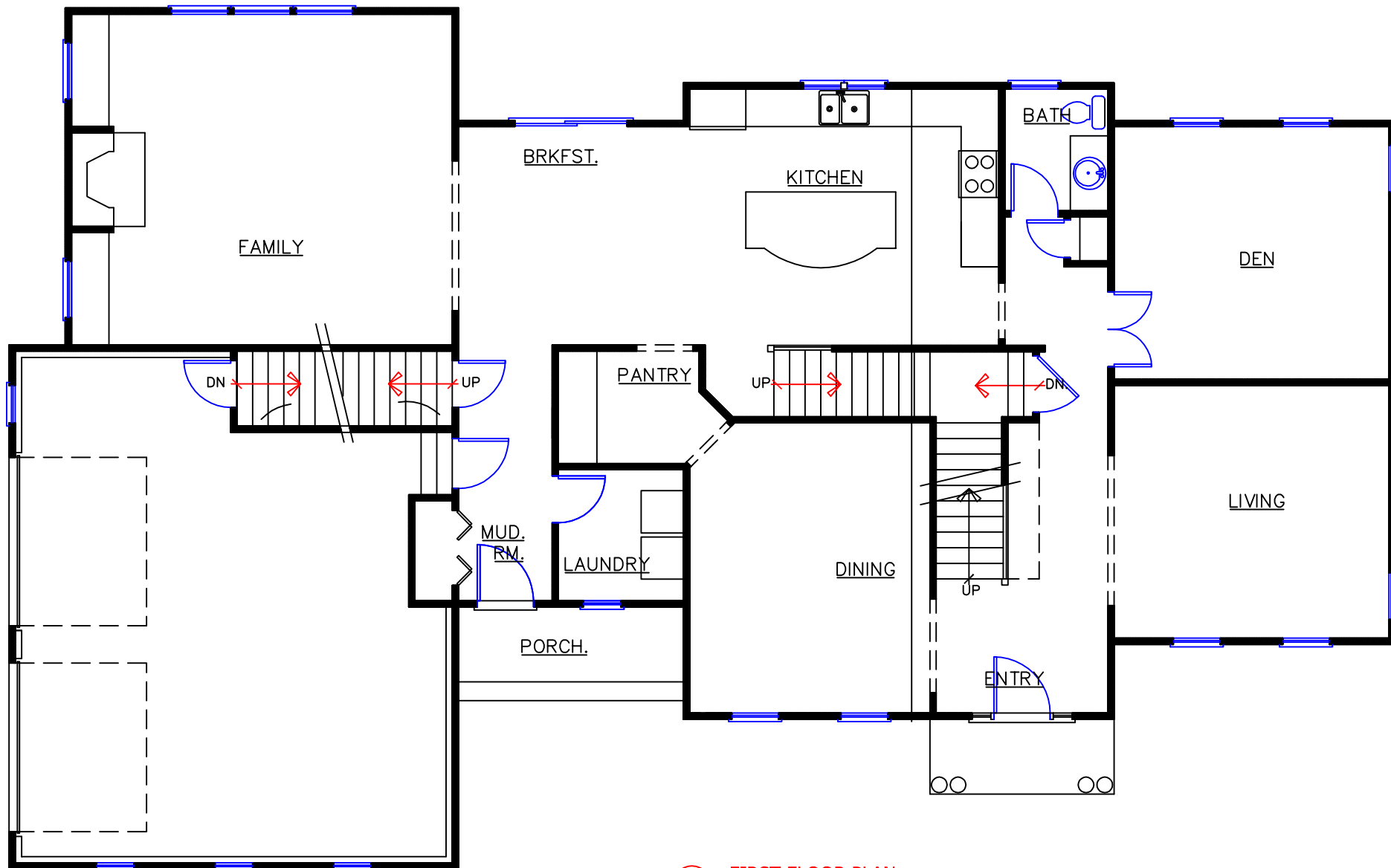
FIRST FLOOR PLAN NTS
